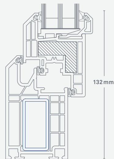
MD-Minergie System
